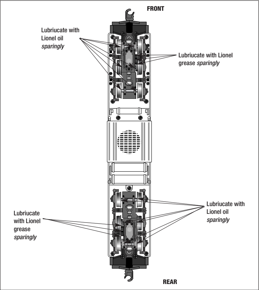
Figure 6. Lubricating the locomotives
